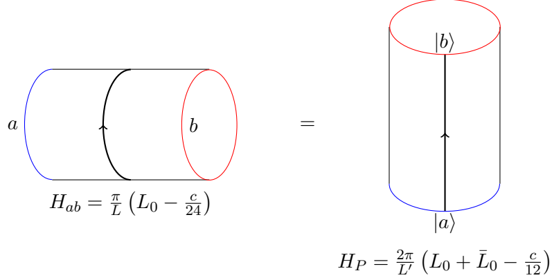
Figure 1.16: Open (left) and closed (right) channels. Arrows indicate the direction of imaginary time.
